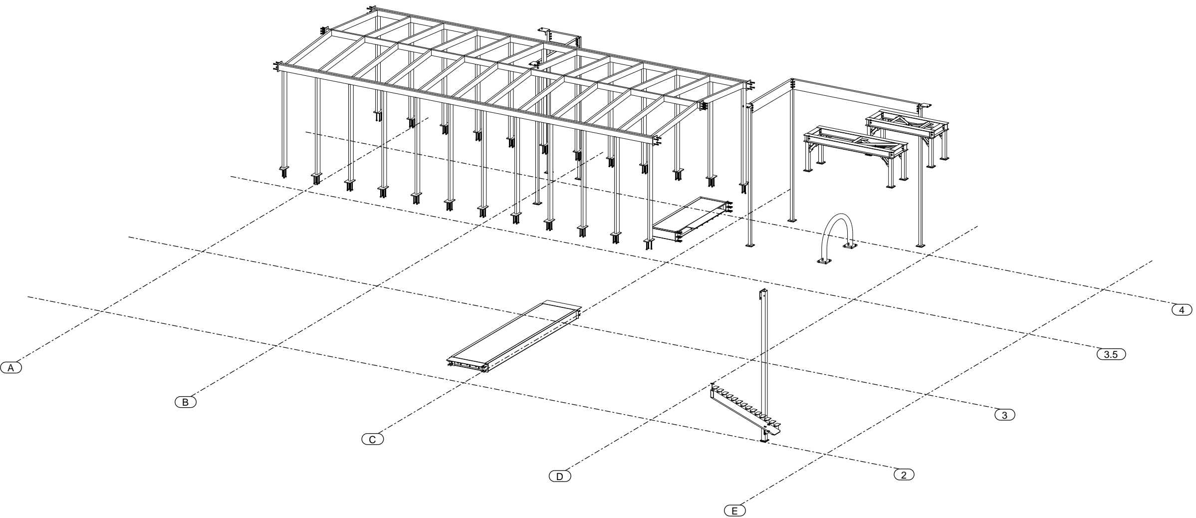
ISOMETRIC VIEW F.D.N.Y NEW FIREHOUSE
